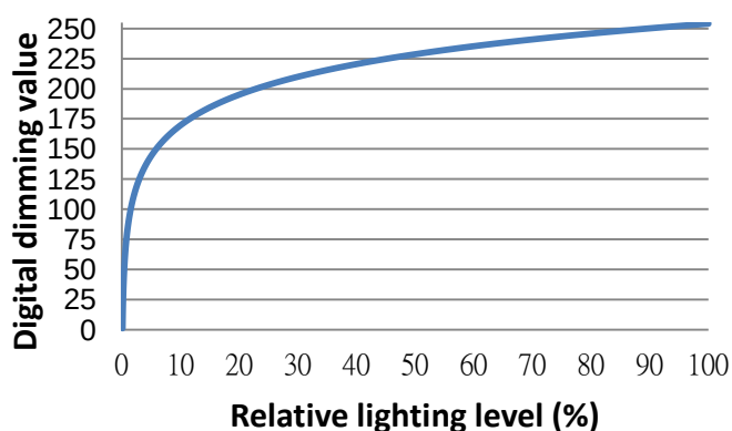
Dimming characteristics
